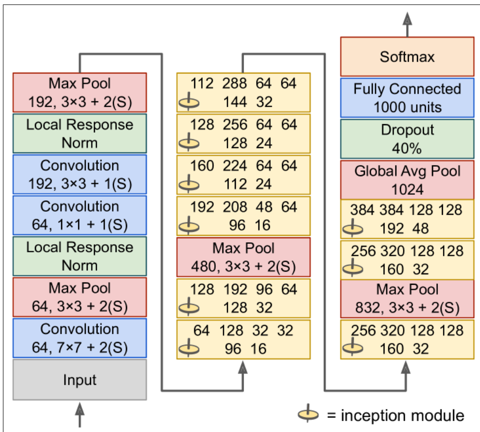
Figure 14-14. GoogLeNet architecture
